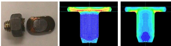
Reduced Strains with Redesigned Process
