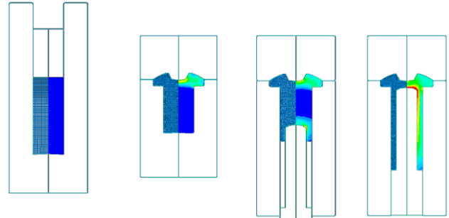
Simulation of Forming Sequence of a Rivet
